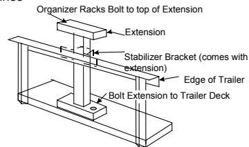
Mounting on trailers with round & angle sides. Extensions can be used to ensure stable (Figure 1)
